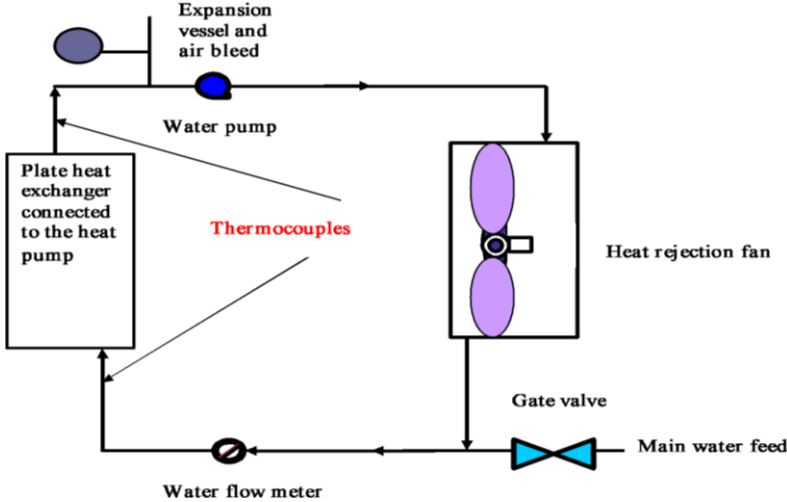
Figure 1. Sketch of installing heat pump.
