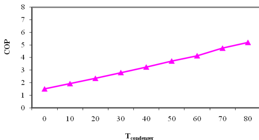
Figure 7. Heat pump performance vs condensation temperature.
