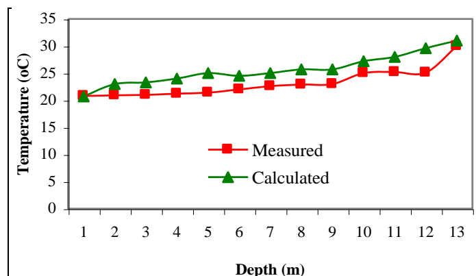
Figure 12. Comparison of calculations and experiments for unsaturated soil without groundwater flow (US).
