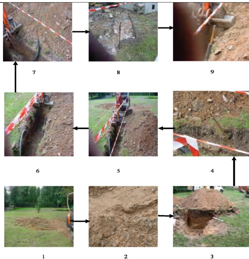
Figure 3. Showing the drilling (1-2) digging of the pit (3), connection of the manifolds (4), grouting, preparation of the coils (5-6) and the source loop, which consists of two earth loops: one for vapour and one for liquid (7-9).
