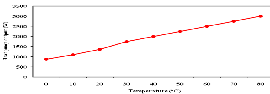
Figure 20. Variation of heat pump output with temperature.
