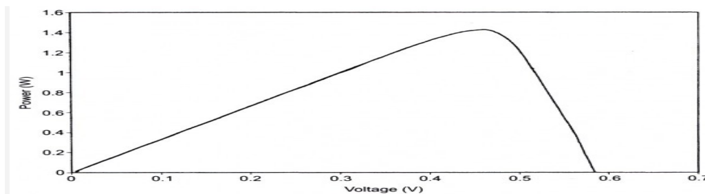
Figure 2.1 Typical power output Vs voltage of silicon PV cell (ITACA, nd)
