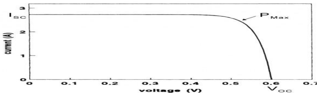
Figure 2.2: Typical I-V graph of silicon PV cell (ITACA, nd)
