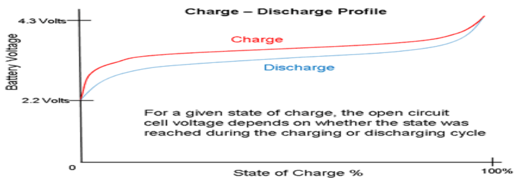
Figure 2.3: Charge-discharge profile of a rechargeable battery (2005)
